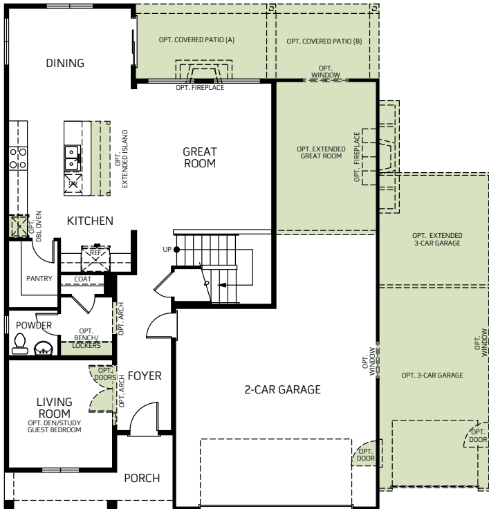
FIRST FLOOR 1,118 Sq. Ft.
