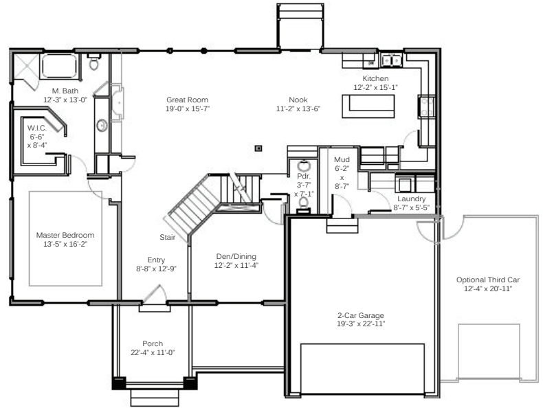
MAIN FLOOR
