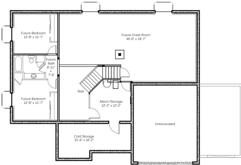
BASEMENT FLOOR
