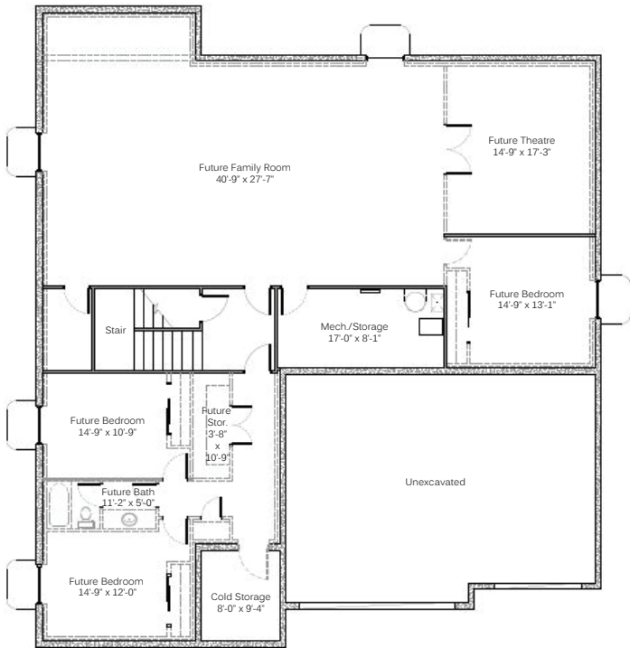
BASEMENT FLOOR
