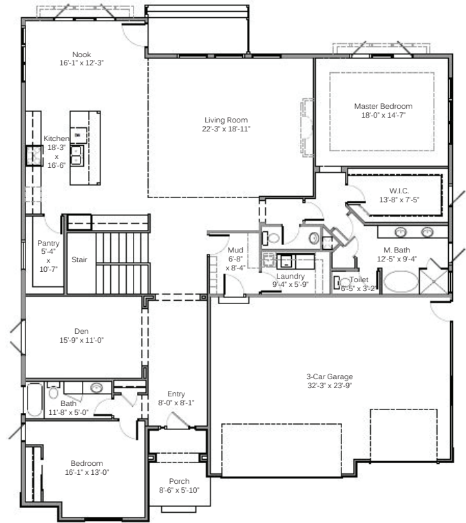
MAIN FLOOR
